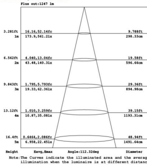
Illuminance Photo-Goniophotometer Method
